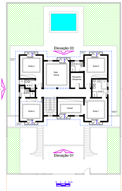
Superior A = 169,48 m 2
